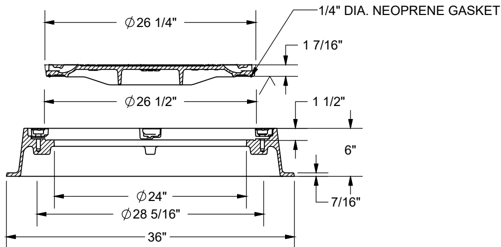
SECTION A-A WATERTIGHT SECTION
