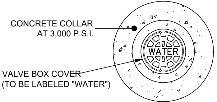
PLAN VIEW FOR UNPAVED AREAS
