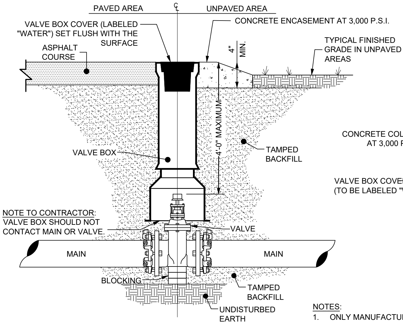
SECTION VIEW
